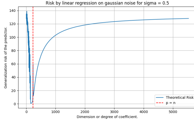
Figure 5.4: Similar experiment according to setting and result of Theorem 5.5, where p is in the range [1, 5523] . Here, we can see small double descent modelled exactly at the interpolation threshold, while the later region exhibit similar phenomenon as bias-variance tradeoff.
