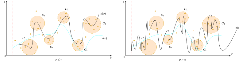
Figure 5.7: Intuition of Hypothesis 5.2.1. Effectively, in the overparameterized range ( p > n ), the problem turns into soft interpolation, where the polynomial is possible to be dense enough such that relative error remains internally low. This can also happen if the dataset itself is intrinsically large.
