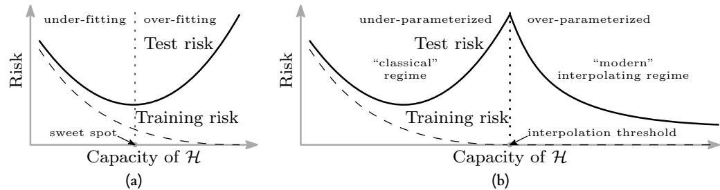
Figure 1. Curves for training risk (dashed line) and test risk (solid line). (a) The classical U-shaped risk curve arising from the bias-variance trade-off. (b) The double descent risk curve , which incorporates the U-shaped risk curve (i.e., the “classical” regime) together with the observed behaviour from using high capacity function classes (i.e., the “modern” interpolating regime), separated by the interpolation threshold. The predictors to the right of the interpolation threshold have zero training risk. Reproduced from Belkin et al. 2019a.
