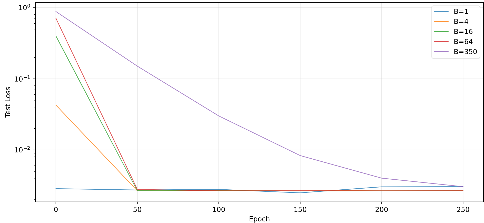
Training Trajectories: k=15 ( \gamma=1.5 )
