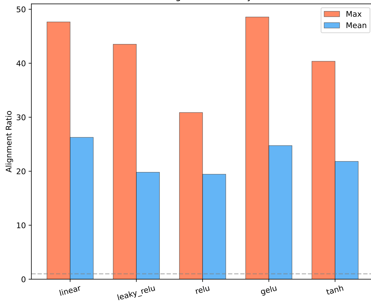
Max & Mean Alignment Ratio by Activation
