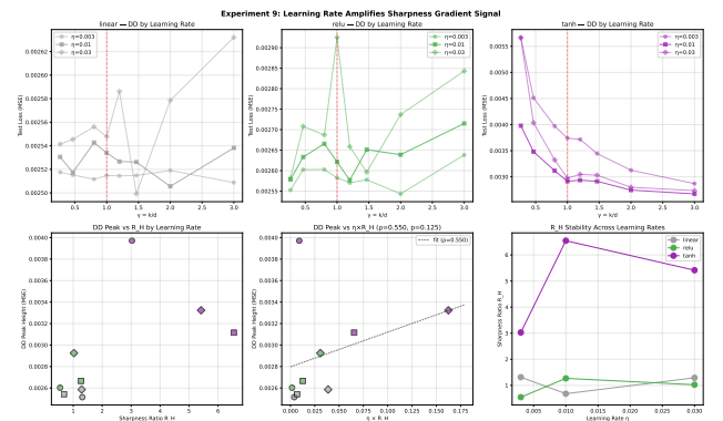
Figure 10. Learning rate modulation of the sharpness ratio. (Top) Double descent curves at three learning rates. (Bottom left) DD peak vs. R_H by \eta . (Bottom center) DD peak vs. \eta \times R_H combined metric ( \rho = 0.550 , n = 9 ). (Bottom right) Stability of R_H across learning rates ( \text{CV} \approx 0.3 ).
