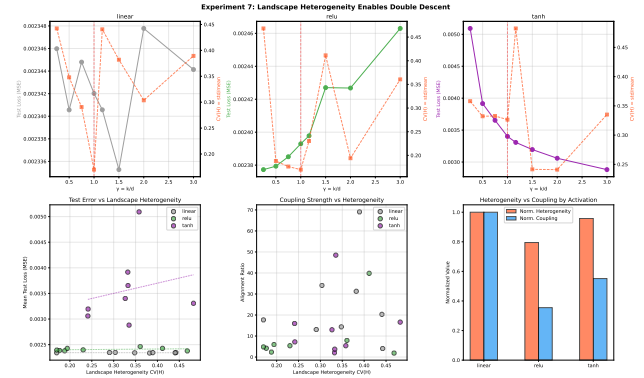
Figure 8. Landscape heterogeneity across activations. (Top) Double descent curves and Hessian trace CV for each activation. (Bottom left) Test error vs. \text{CV}(H) , showing positive correlation. (Bottom right) Normalized heterogeneity vs. coupling strength.
