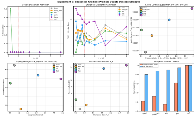
Figure 9. Sharpness Ratio as predictor of double descent. (Top left) Double descent curves for five activations. (Top center) \text{Tr}(H) vs. \gamma on log scale, revealing the sharpness differential. (Top right) DD peak height vs. R_H (Spearman \rho = 0.700 , n = 5 ). (Bottom) Additional diagnostics: coupling vs. R_H , recovery rate, and normalized bar comparison.
