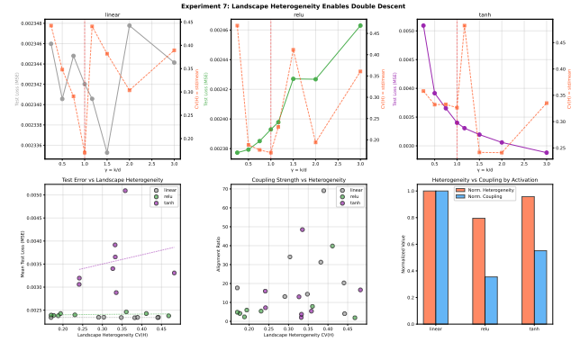
Figure 8. Landscape heterogeneity across activations. (Top) Double descent curves and Hessian trace CV for each activation. (Bottom left) Test error vs. CV(H), showing positive correlation. (Bottom right) Normalized heterogeneity vs. coupling strength.
