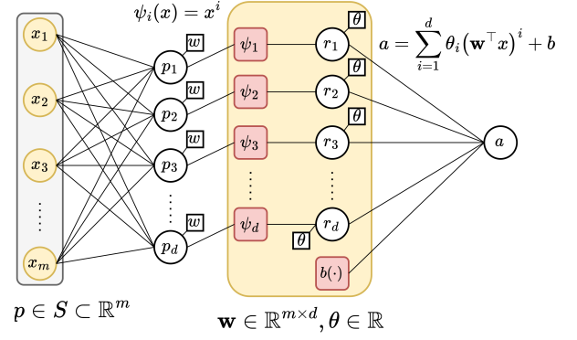
Figure 15. Illustration of polynomial model in definition 9.7.
