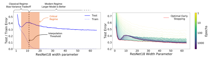
Figure 6. Left: Train and test error as a function of model size, for ResNet18s of varying width on CIFAR-10 with 15% label noise. Right: Test error, shown for varying train epochs. All models trained using Adam for 4K epochs. The largest model (width 64) corresponds to standard ResNet18. Resued from Nakkiran et al. 2019.
