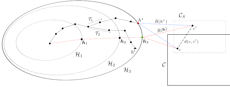
Figure 16. Illustrative dynamic of the learning problem. For an incremental hypothesis space sequence \mathcal{H}_1, \mathcal{H}_2, \mathcal{H}_3 , we aim to obtain the procedure \mathcal{T} that would either reach the generalization solution h , or the empirical solution h^* for a particular hypothesis class, with respect to the concept c and its observed concept c' . Model selection hence dictates how an algorithm or procedure than choose the best possible hypothesis to approximate the generalization solution from the empirical solution set. Do notice that here we explicitly state that the data would create a proxy concept that overlaps with the concept class and of some arbitrary ‘distance’ from the true concept by d(c, c') . In case the two classes overlap, there still exists the arbitrary distance. Also, we can also observe the intuitive notion of increasing hypothesis class - while it indeed can help in getting closer to the concept class, the somewhat intrinsic property of current learning theory being the relative random procedure class make it probabilistically unstable.
