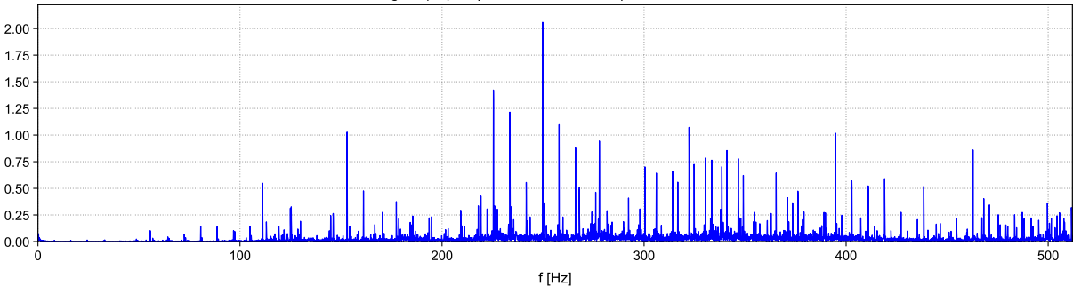
timesignal (21).uff | 6- 3-2026 10: 9:33 | Native Acceleration
