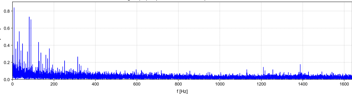
timesignal (45).uff | 6- 3-2026 10:29:10 | Native Acceleration
