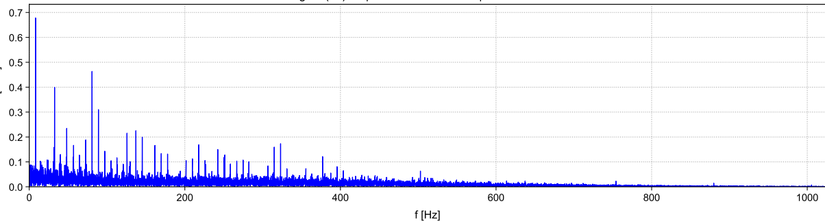
timesignal (56).uff | 6- 3-2026 10:39:19 | Native Acceleration
