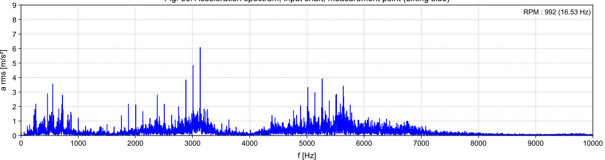
Fig. 30: Acceleration spectrum, input shaft, measurement point (Lifting side)
