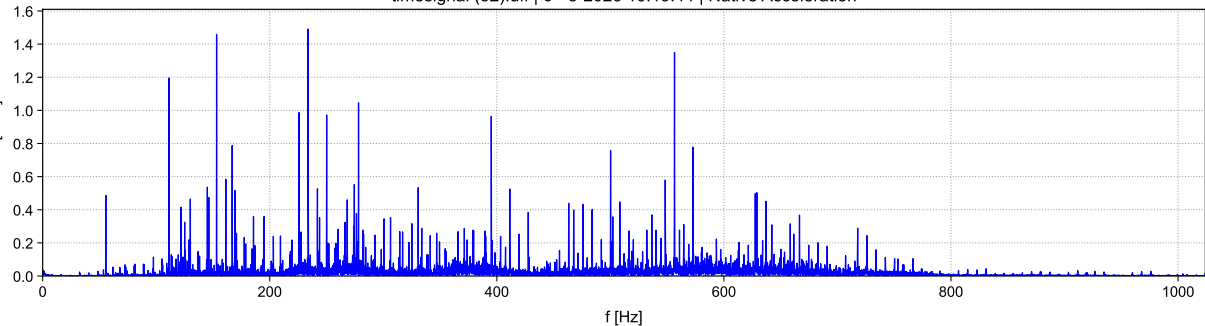
timesignal (32).uff | 6- 3-2026 10:19:44 | Native Acceleration
