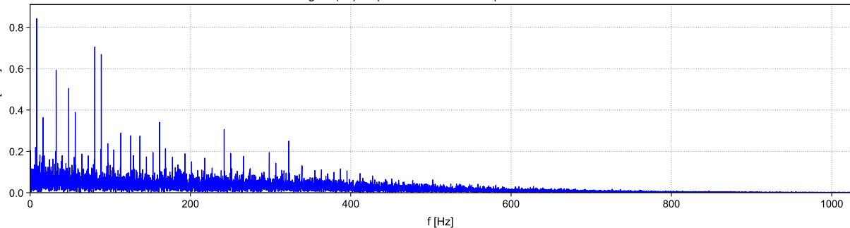
timesignal (36).uff | 6- 3-2026 10:18:47 | Native Acceleration
