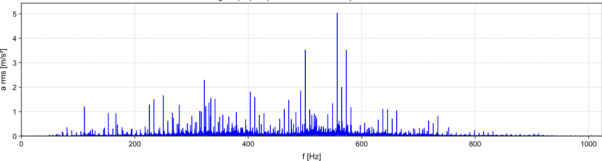
timesignal (37).uff | 6- 3-2026 10:25:52 | Native Acceleration
