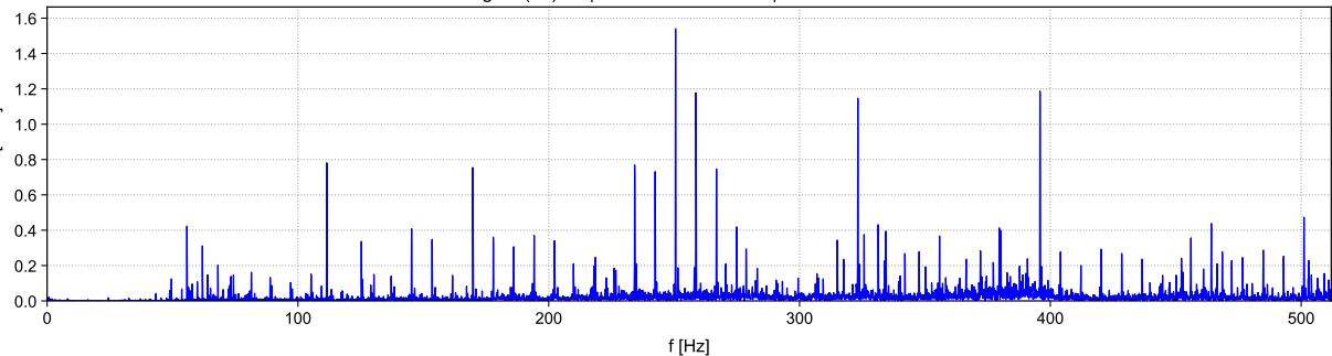
timesignal (48).uff | 6- 3-2026 10:36:59 | Native Acceleration
