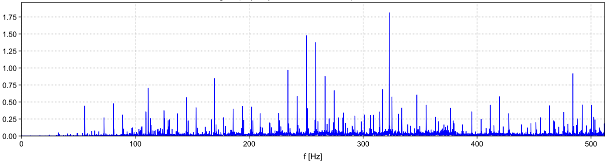
timesignal (53).uff | 6- 3-2026 10:41:33 | Native Acceleration
