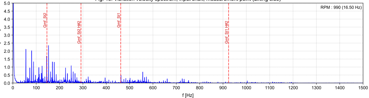
Fig. 18: Vibration velocity spectrum, input shaft, measurement point (Lifting side)
