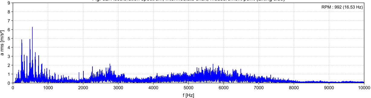
Fig. 32: Acceleration spectrum, intermediate shaft, measurement point (Lifting side)
