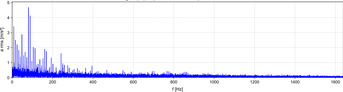
timesignal (19).uff | 6- 3-2026 10: 1: 9 | Native Acceleration
