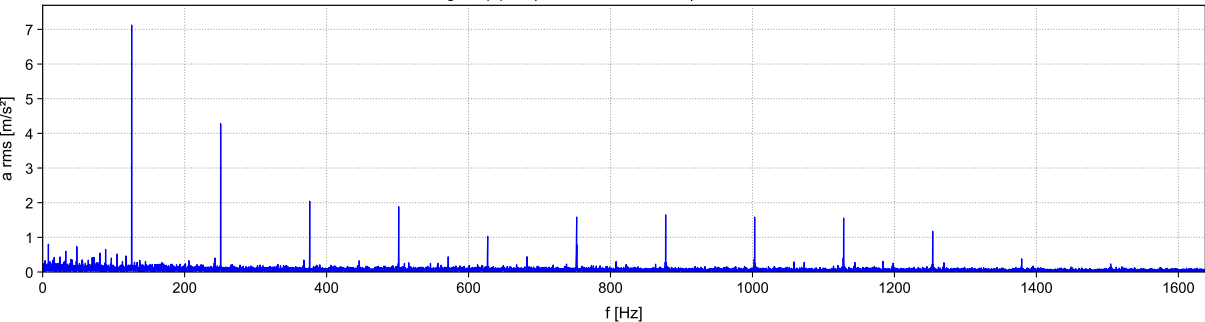
timesignal (3).uff | 6- 3-2026 9:48: 0 | Native Acceleration
