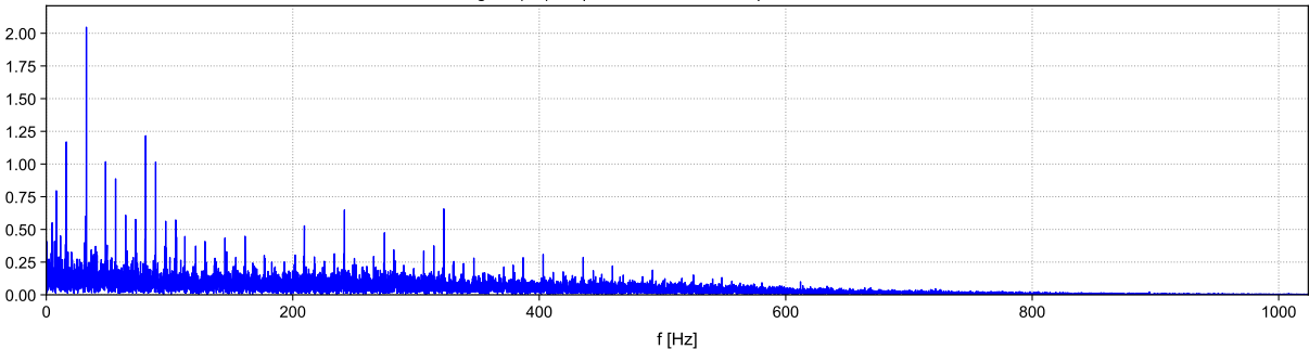
timesignal (31).uff | 6- 3-2026 10:12: 7 | Native Acceleration
