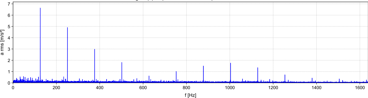
timesignal (4).uff | 6- 3-2026 9:48:39 | Native Acceleration
