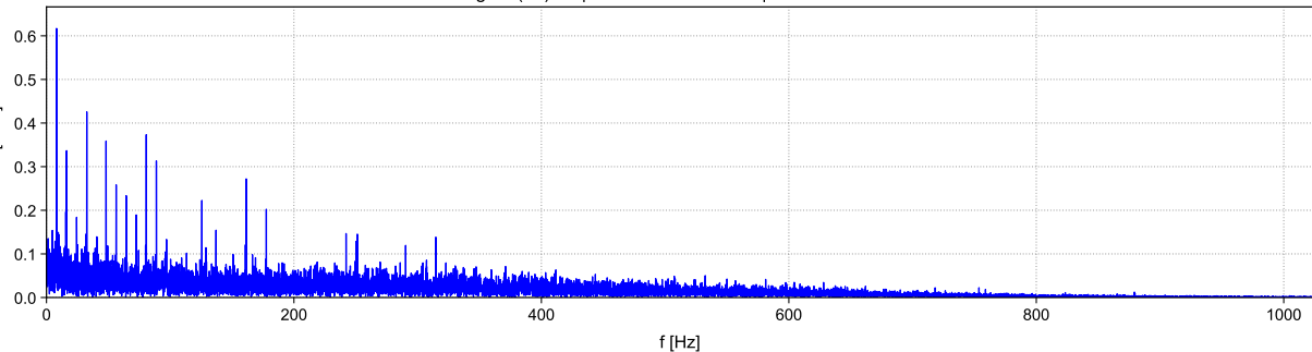
timesignal (46).uff | 6- 3-2026 10:30:10 | Native Acceleration
