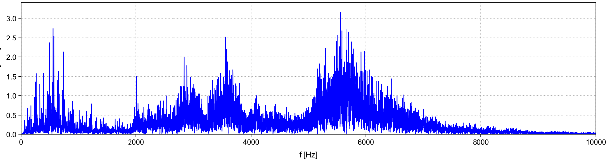
timesignal (49).uff | 6- 3-2026 10:35: 1 | Native Acceleration
