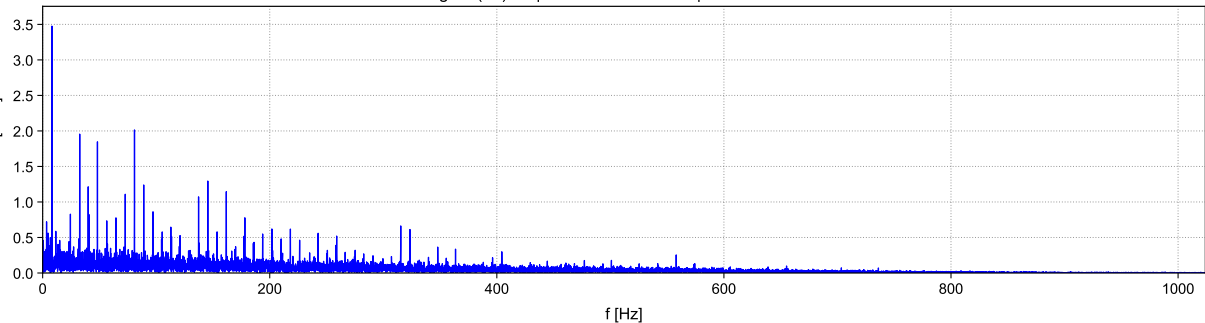
timesignal (51).uff | 6- 3-2026 10:34: 3 | Native Acceleration
