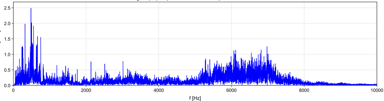
timesignal (54).uff | 6- 3-2026 10:39:39 | Native Acceleration
