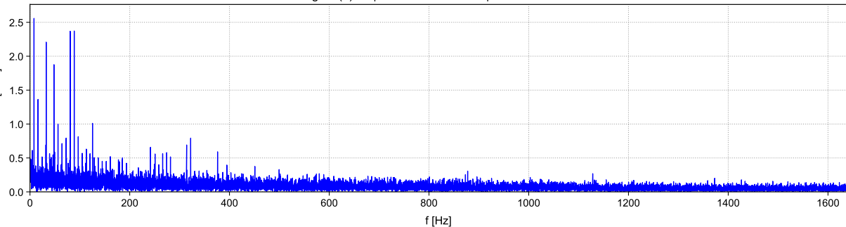
timesignal (8).uff | 6- 3-2026 9:53:30 | Native Acceleration
