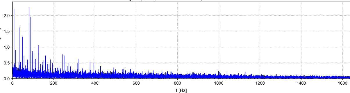
timesignal (9).uff | 6- 3-2026 9:52:48 | Native Acceleration
