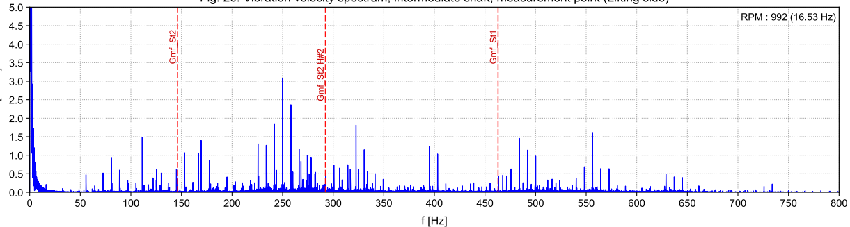
Fig. 20: Vibration velocity spectrum, intermediate shaft, measurement point (Lifting side)
