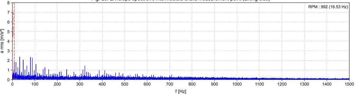
Fig. 26: Envelope spectrum, intermediate shaft, measurement point (Lifting side)
