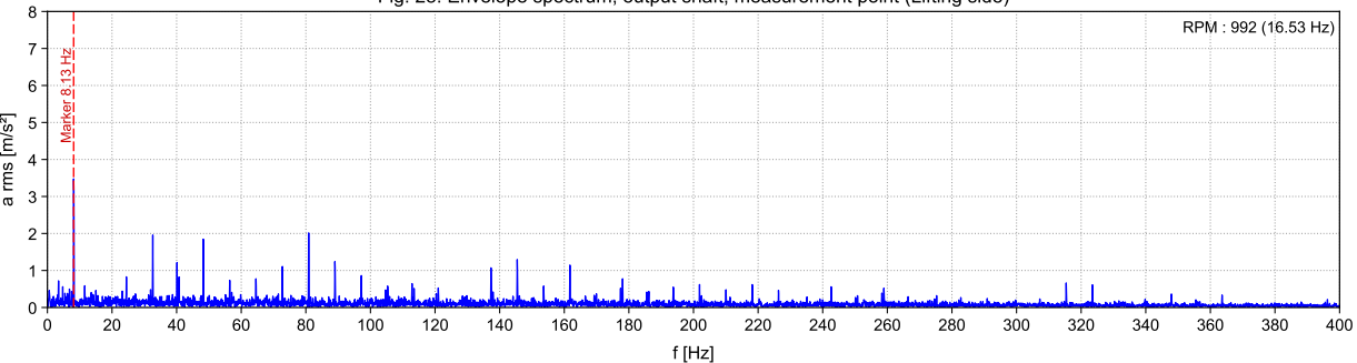
Fig. 28: Envelope spectrum, output shaft, measurement point (Lifting side)
