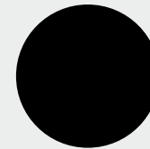
BLACK ANODIZED
