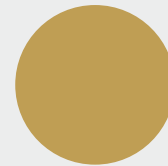
GOLD ANODIZED
