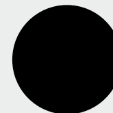
BLACK ANODIZED
