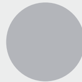
GREY ANODIZED
