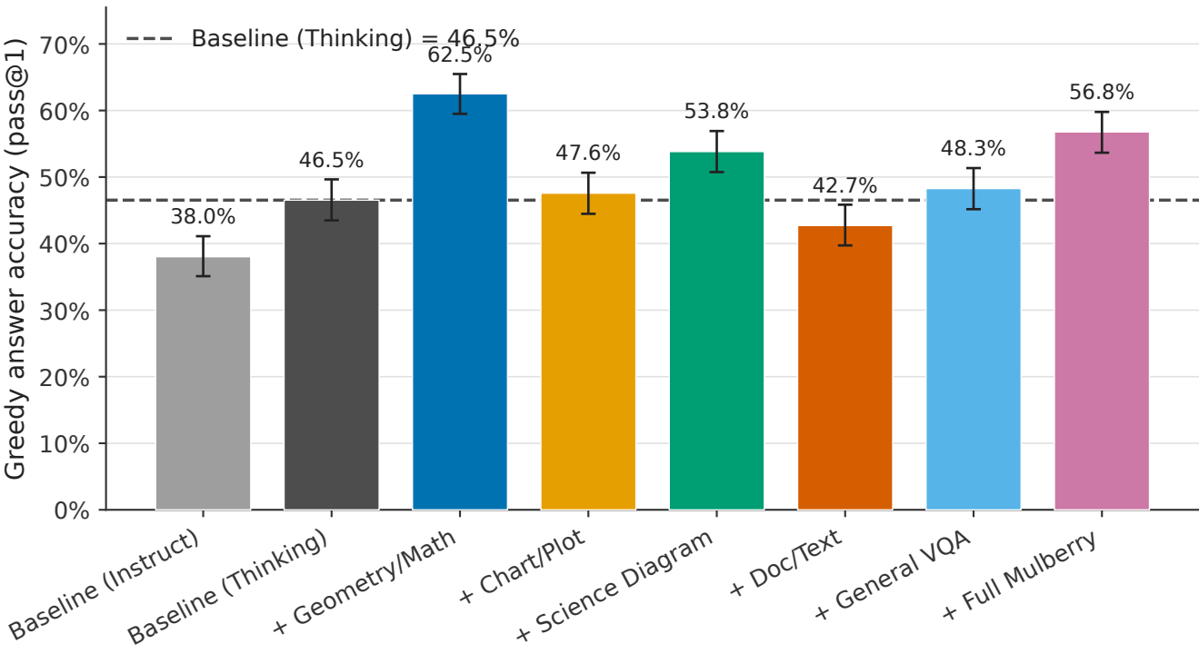
Overall SURDS val_1k accuracy per model (n=1001, Wilson 95% CI)
