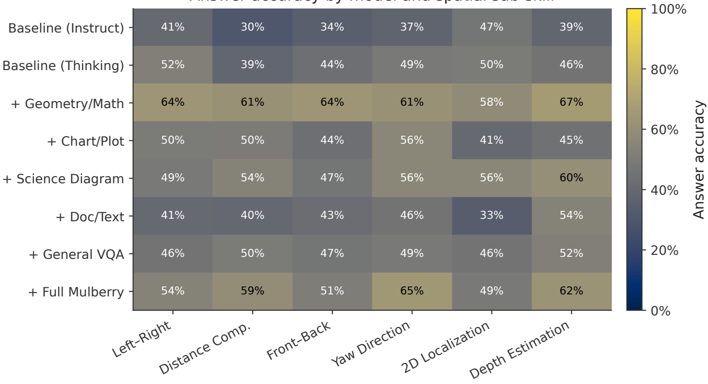
Answer accuracy by model and spatial sub-skill
