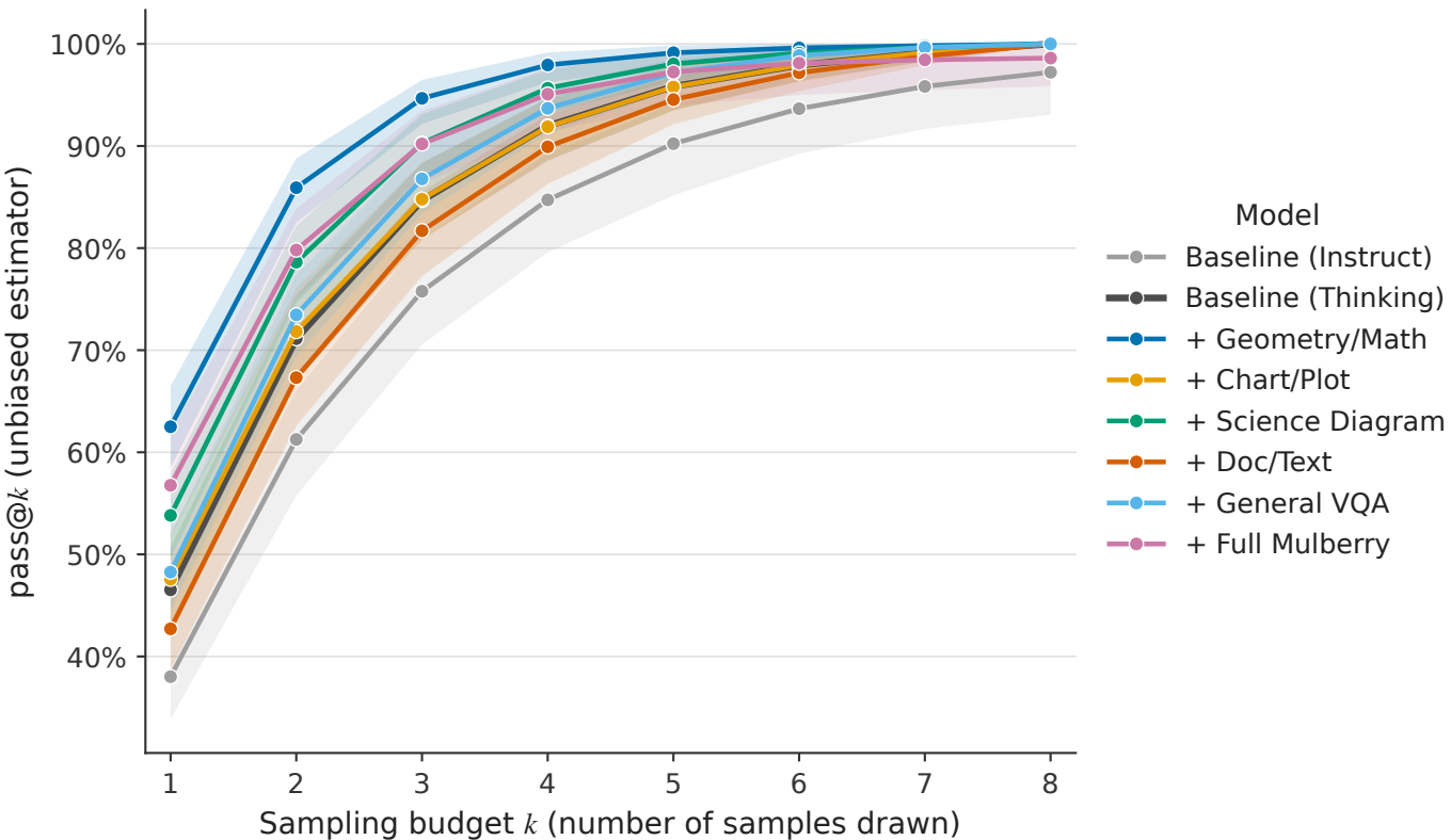
pass@ k scaling per model (SURDS val_1k overall, bootstrap 95% CI)
