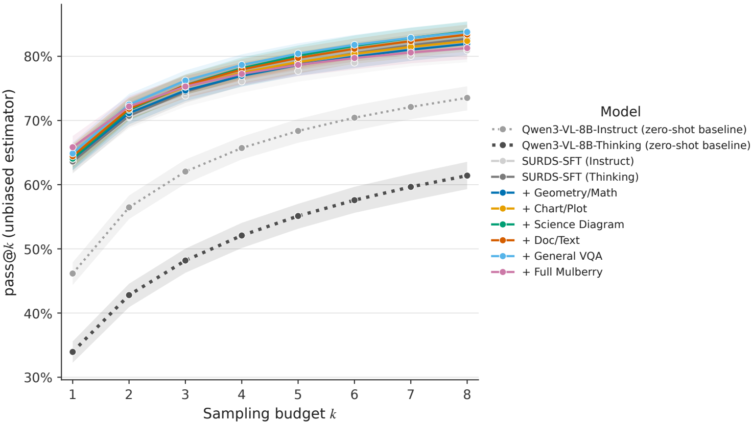
Held-out pass@ k scaling per model (bootstrap 95% CI)
