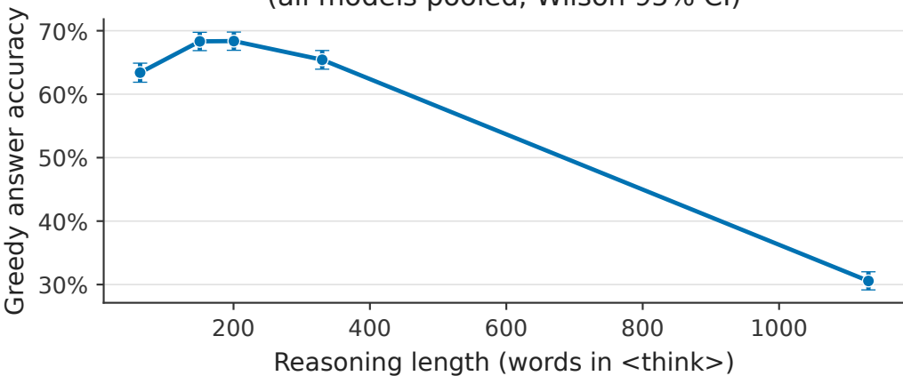
(a) Accuracy vs reasoning length (all models pooled, Wilson 95% CI)
