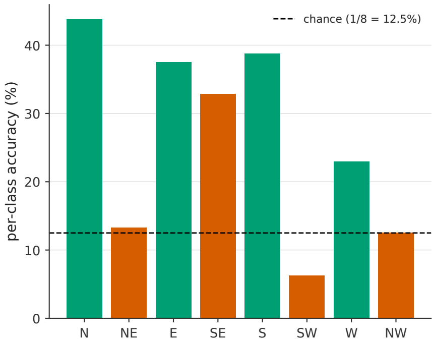
Prediction mass piles onto SE / SW / S Diagonals NE/SW/NW at-or-below chance — SE inflated by the over-prediction
