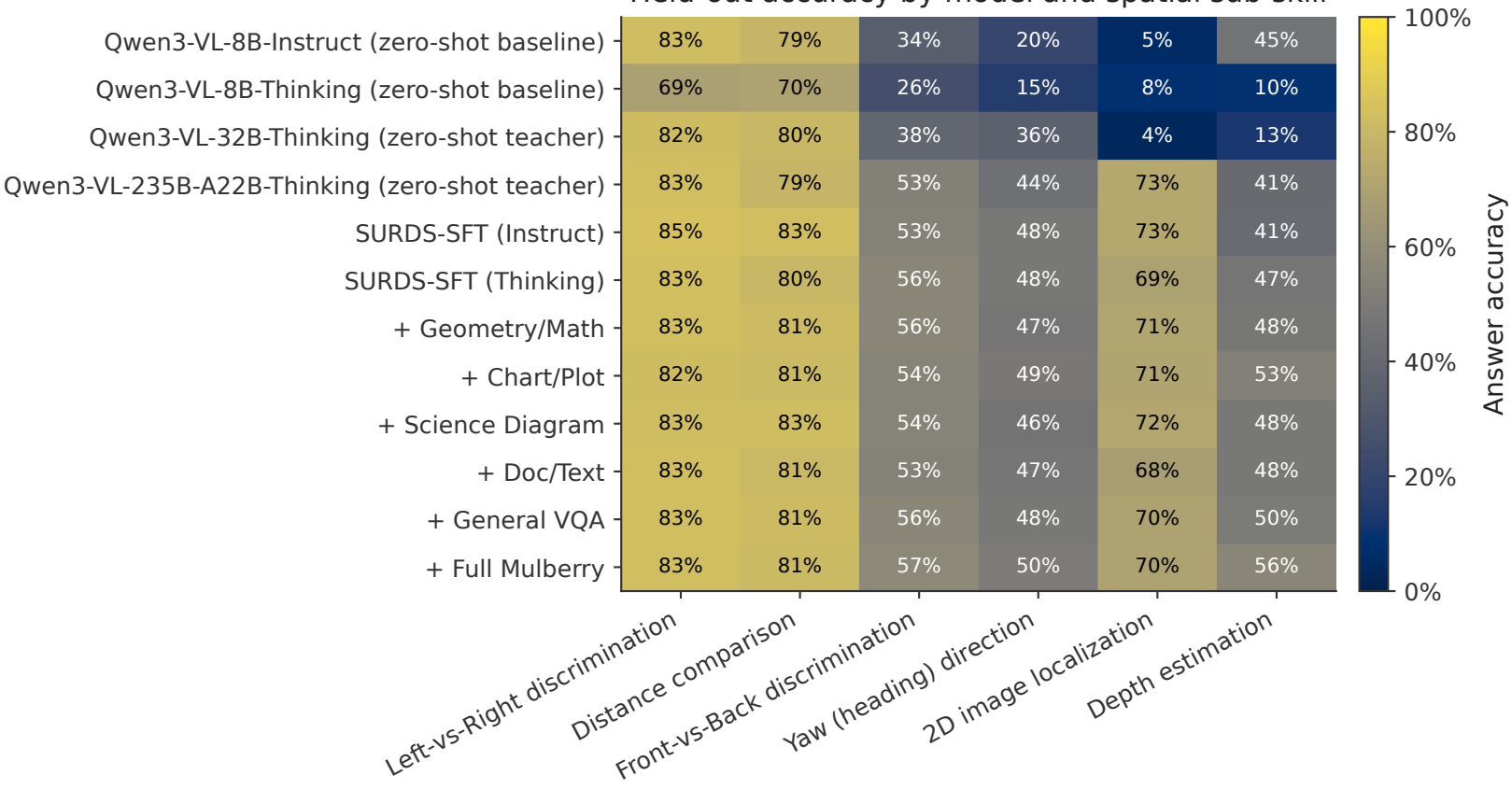
Held-out accuracy by model and spatial sub-skill
