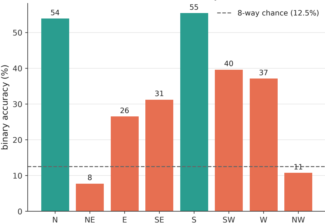
Per-class accuracy
