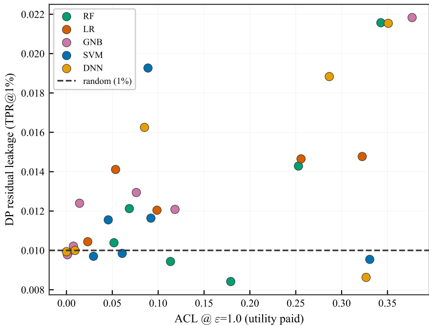
Utility paid \neq protection gained ( \rho=0.42 , n=30 )
