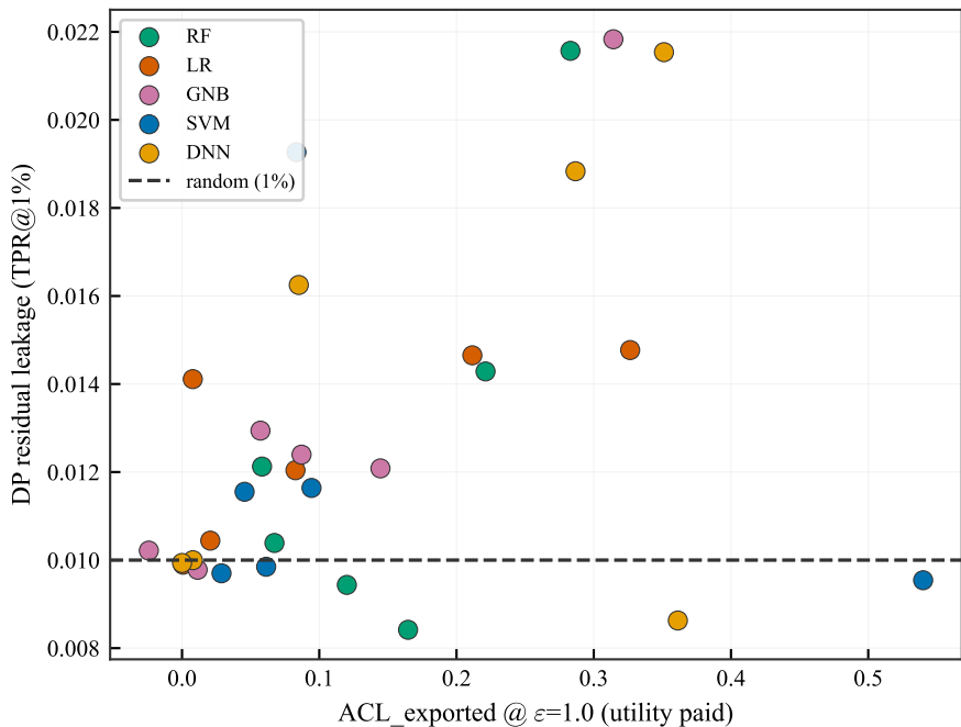
Utility paid \neq protection gained ( \rho=0.31 , n=30 )
