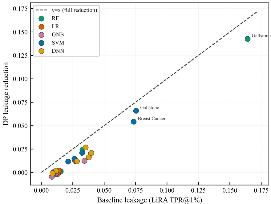
DP benefit scales with baseline leakage ( \rho=0.89 )
