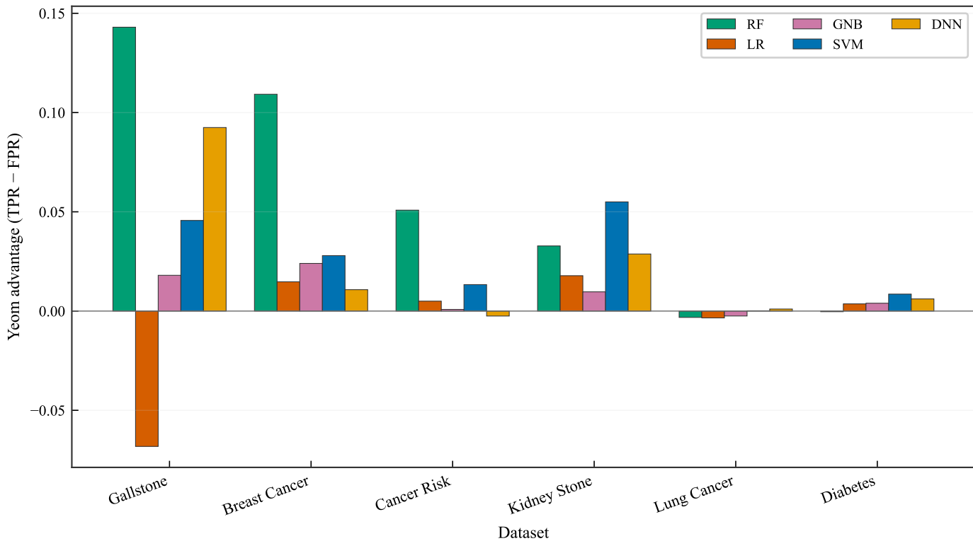
Baseline average-case leakage (Yeom advantage)
