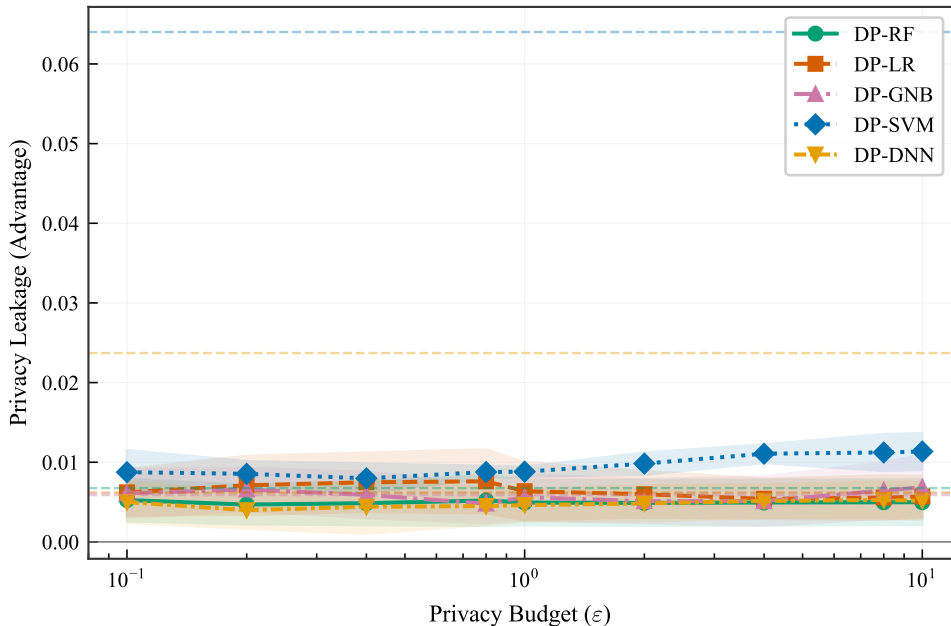
Privacy Leakage — Diabetes ( N=70,692 )
