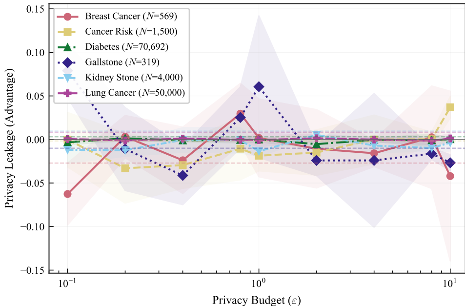
Privacy Leakage — DP-GNB
