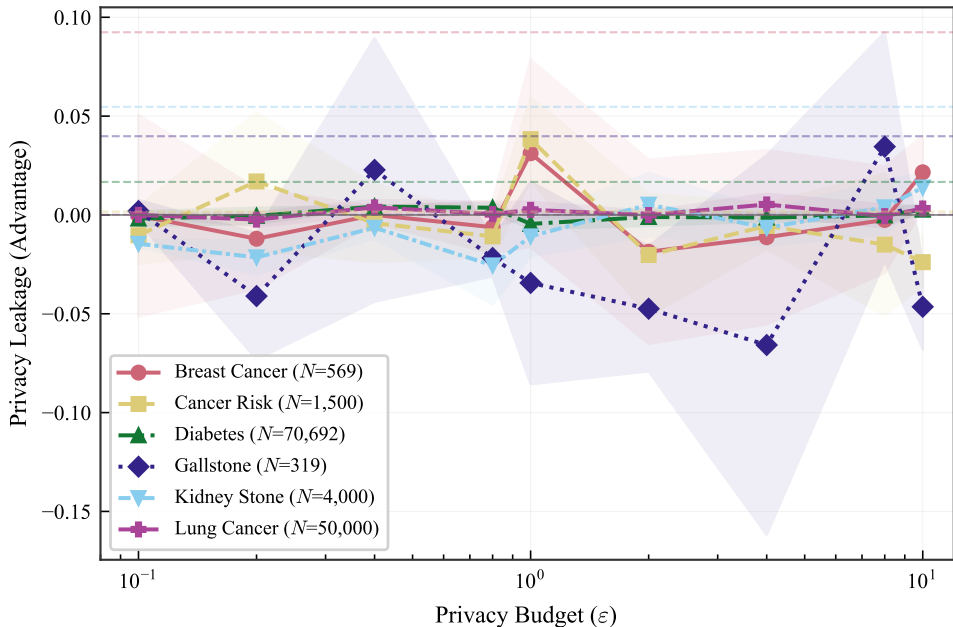
Privacy Leakage — DP-SVM
