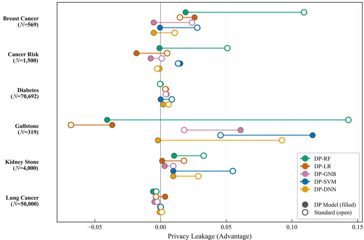
Privacy Leakage: Standard (open) vs DP (filled) at \epsilon=1.0
