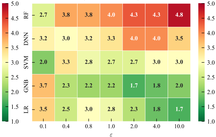
(b) Average Rank by \epsilon (1 = Best, 5 = Worst)
