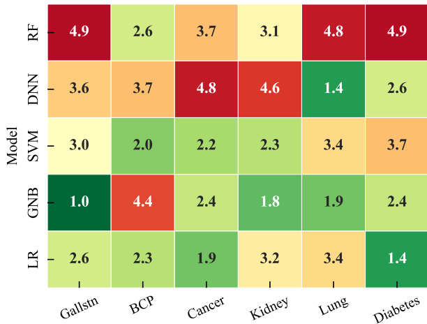
(a) Average Rank by Dataset (1 = Best, 5 = Worst)
