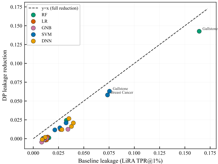
DP benefit scales with baseline leakage ( \rho=0.91 )
